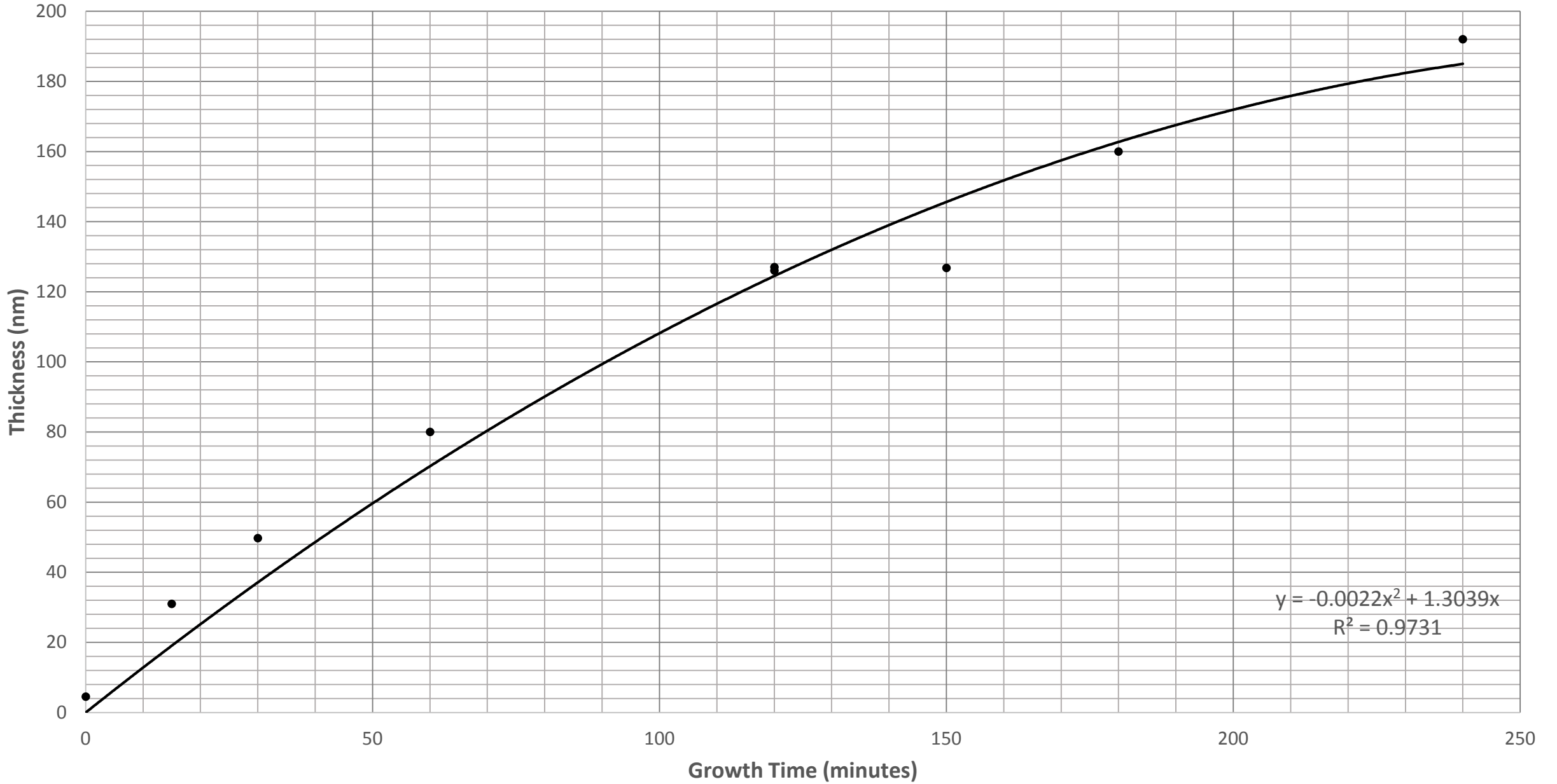
CVD 1034 Dry Oxidation Growth Thickness at 1050 deg, n-type, (100) Si
